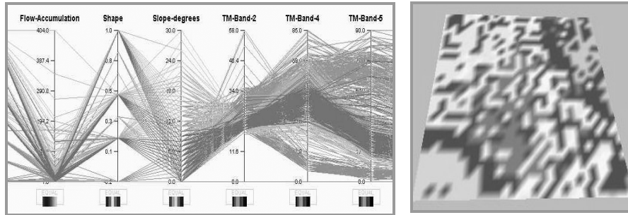
Figure 3. Five candidate categories constructed in a PCP then learned using LVQ.
