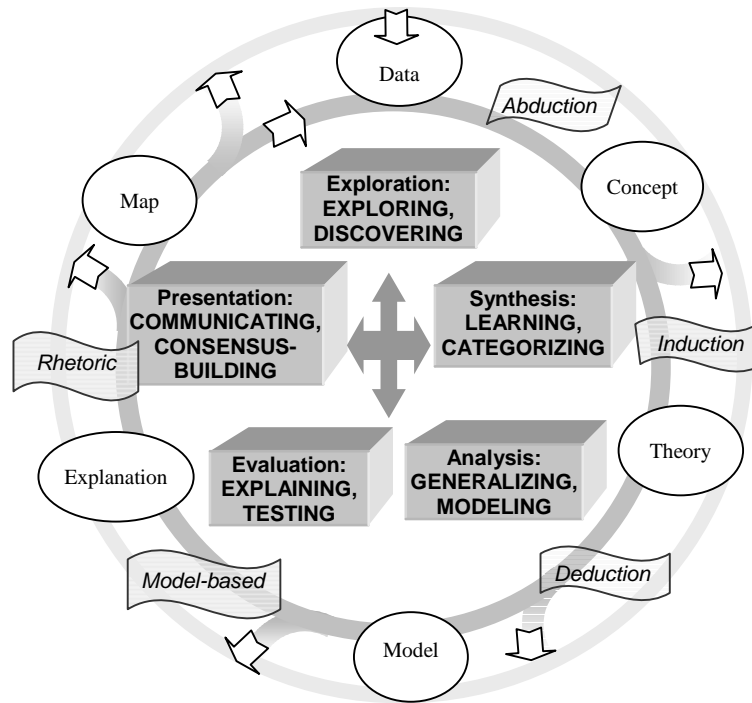
Figure 1: a generalized framework for geoscientific discovery consisting of exploratory, synthesis, analysis, evaluation, and presentation activities. These respectively correlate with the evolution of features, concepts, theories and models, explanations, and presentations.
