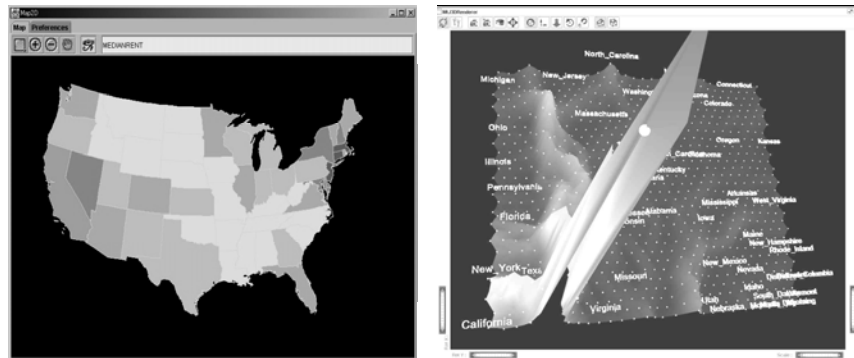
Figure 2. Two views of a demographic dataset, allowing the user to explore the data from a number of different perspectives. Dynamic map (left), and a view of the unsupervised clustering of states provided by the SOM.
